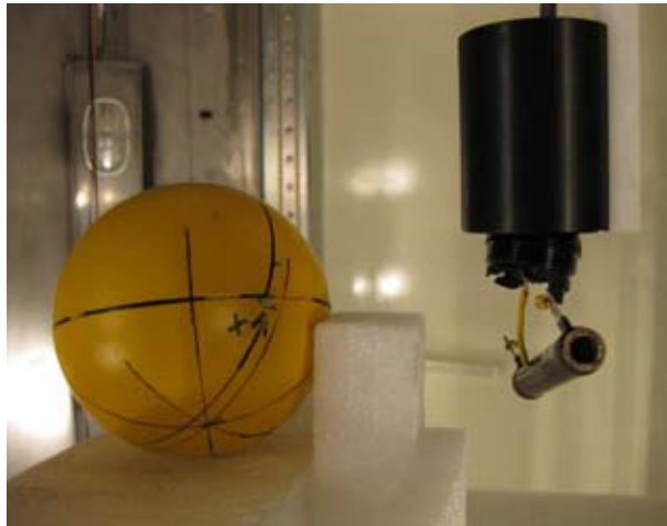
Figure 26: 50 Hz B -field measurement of 4.1\text{ k}\Omega resistor load drawing 12.8 W of power.
